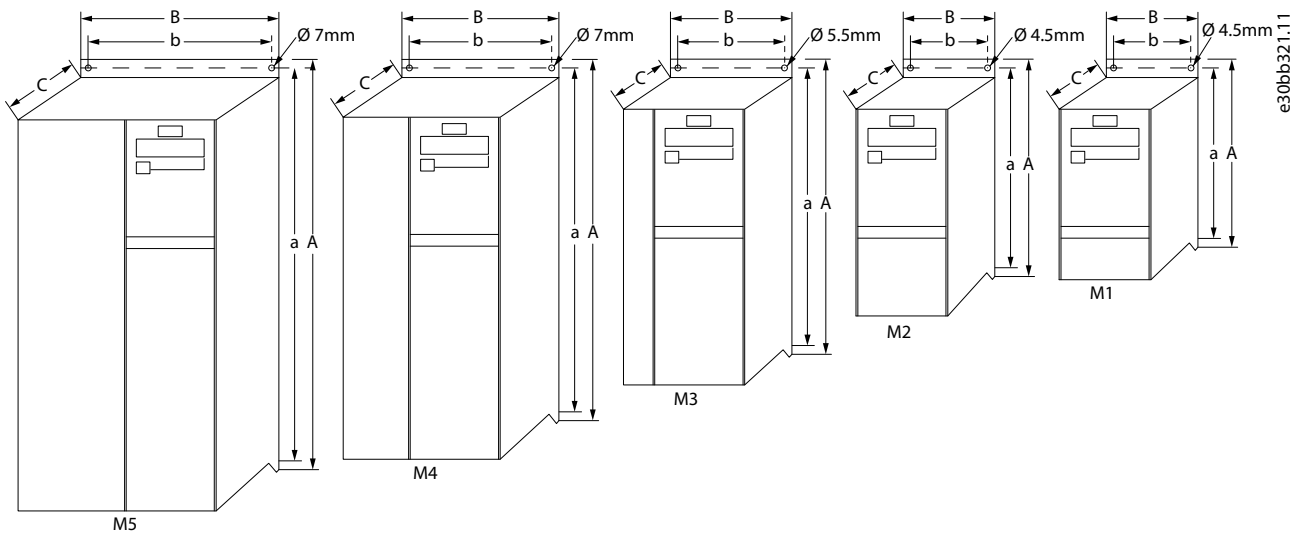
Illustration 1: Mechanical Dimensions
