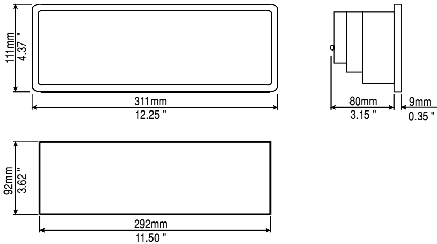
Figure 6 - Dimensions
