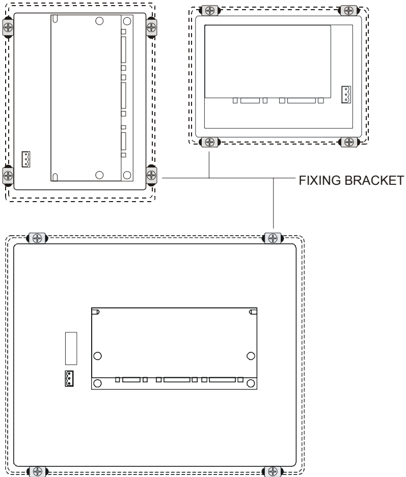
Figure 45 – Fixing bracket position
