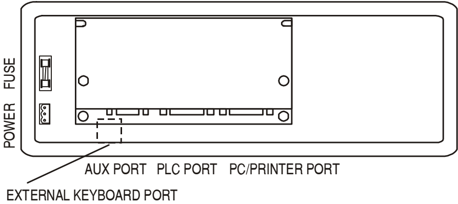
Figure 30 - Connectors
