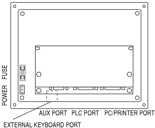
Figure 23 - Connectors
