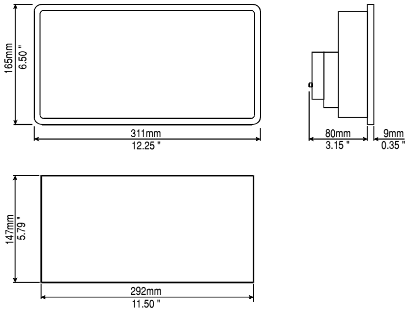
Figure 7 - Dimensions
