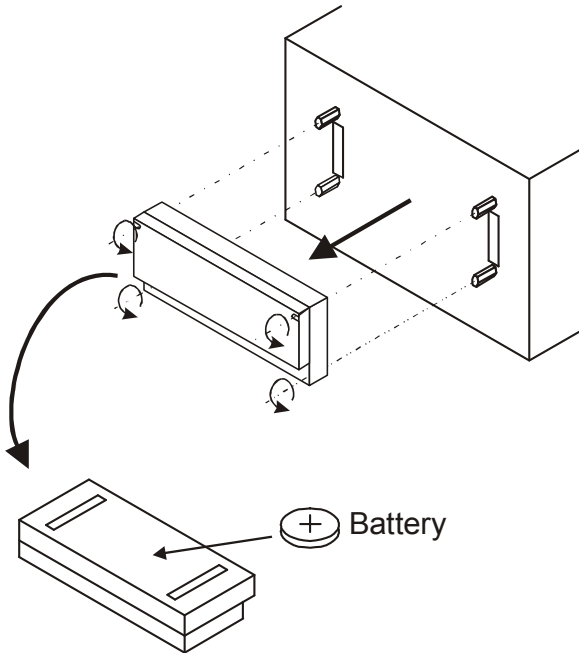
Figure 42 - battery replacement
