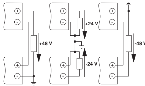
Figure 11 Series operation
