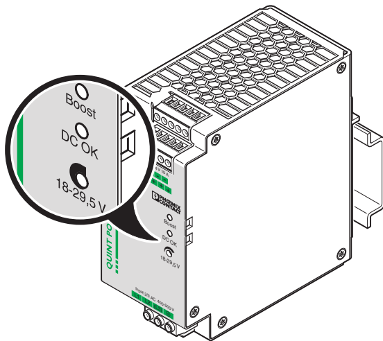
Figure 10 Signal outputs
